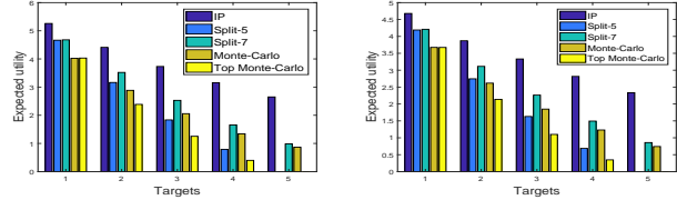
(a) Uniform distribution (b) Exponential distribution
